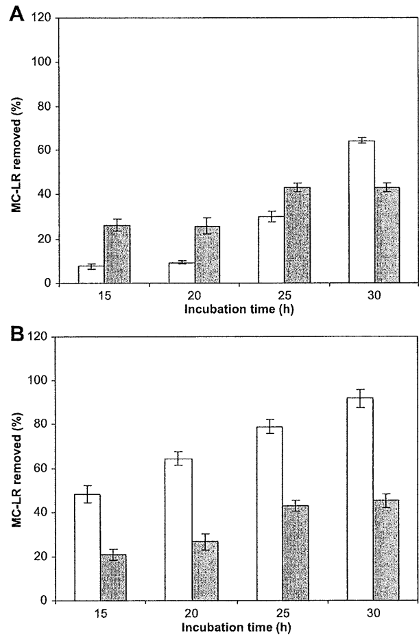
Fig. 2. (A) Microcystin-LR removal percentages by viable cells of Lactobacillus plantarum IS-10506 at pH 7, white bars indicate 22 °C and grey bars 37 °C. Error bars indicate confidence intervals at 95% level. (B) Microcystin-LR removal percentages of viable cells of Lactobacillus plantarum IS-20506 at pH 7, white bars indicate 22 °C and grey bars 37 °C. Error bars indicate confidence intervals at 95% level.
