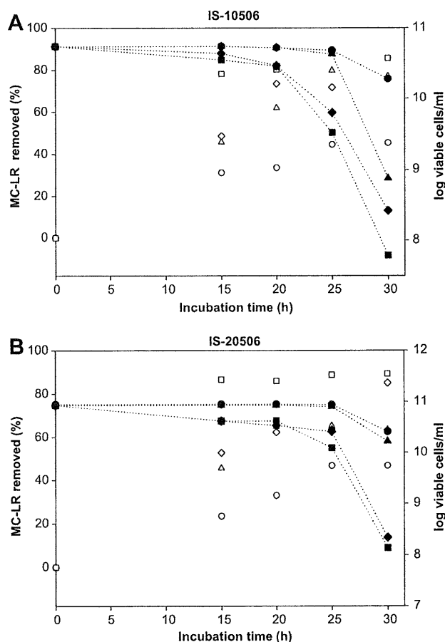
Fig. 3. (A) MC-LR removed (%) and log viable cells/mL of IS-10506 strain at different glucose concentration during incubation at 37 °C. Empty symbols stand for MC-LR removed, and filled symbols for log viable cells. Symbols (○, ●) denote 0% of glucose, (▲, △) 1% of glucose, (◆, ◇) 2% of glucose and (■, □) 3% of glucose. (B) MC-LR removed (%) and log viable cells mL -1 of IS-20506 strain at different glucose concentration during incubation at 37 °C. Empty symbols stand for MC-LR removed, and filled symbols for log viable cells. Symbols (○, ●) denote 0% of glucose, (▲, △) 1% of glucose, (◆, ◇) 2% of glucose and (■, □) 3% of glucose.
